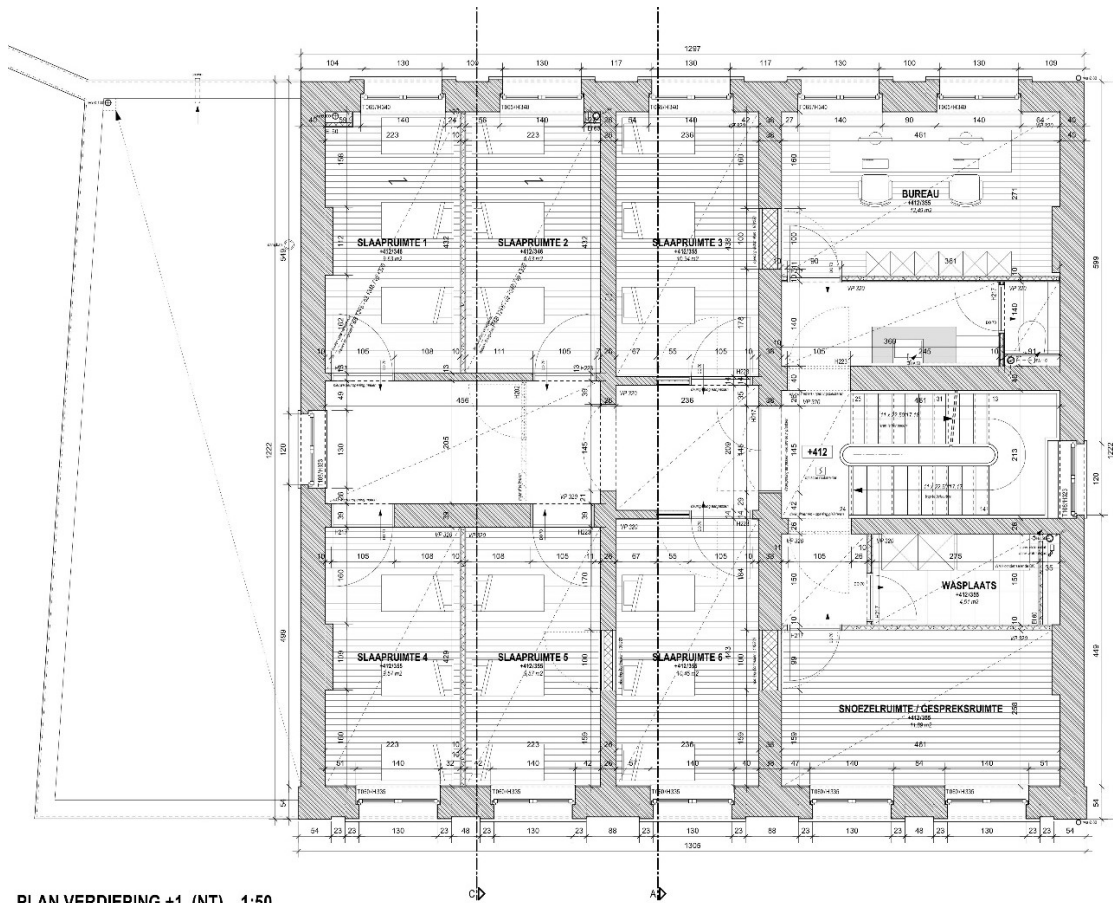
PLAN VERDIEPING +1 (NT) _ 1:50
